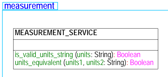
FIGURE 6 rm.support.measurement Package
