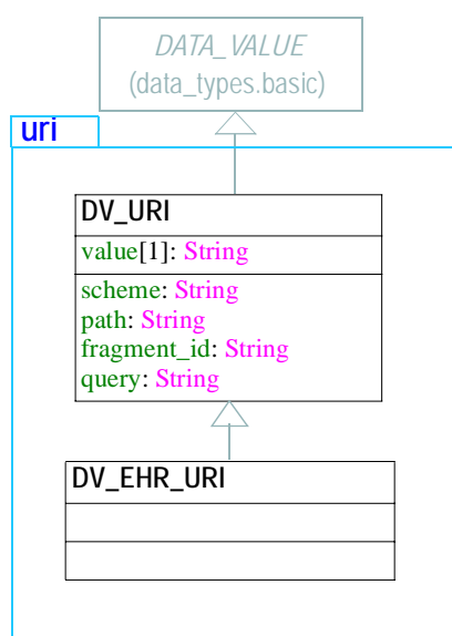
FIGURE 12 rm.data_types.uri Package
