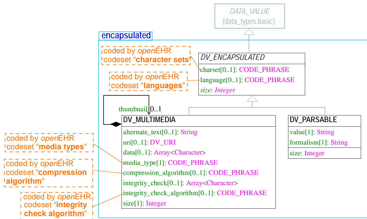
FIGURE 11 rm.data_types.encapsulated Package
